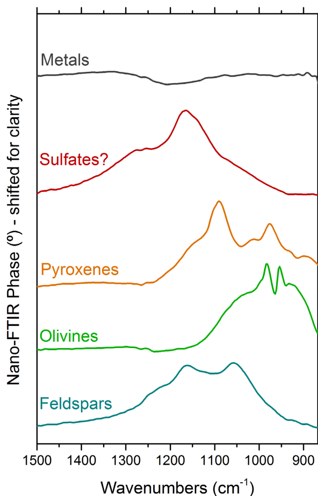
Fig. 8. Average nano-FTIR spectra of minerals and opaque phases observed in the Didim meteorite.
